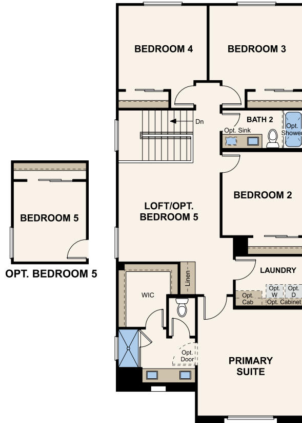
UPPER LEVEL
